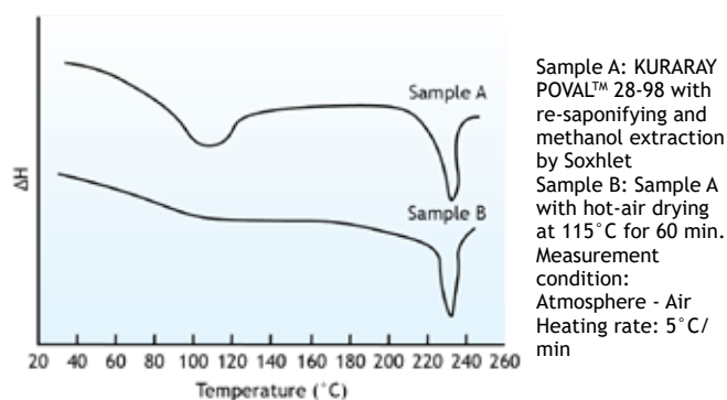
Figure 9. Differential Thermal Analysis Curves of Re-saponified KURARAY POVAL™ 28-98
