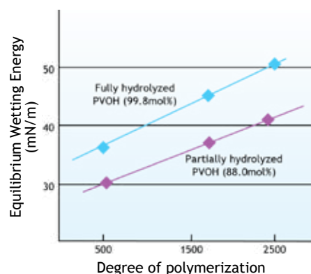
Figure 59. Equilibrium Wetting Energy of PVOH Aqueous Solution
