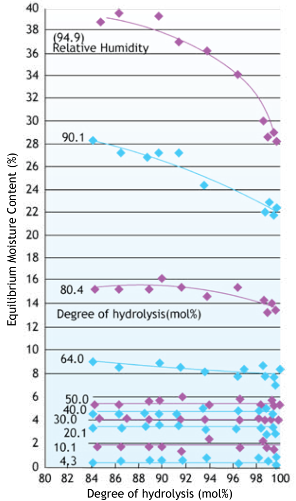
Figure 73. Equilibrium Moisture Content of PVOH Film
