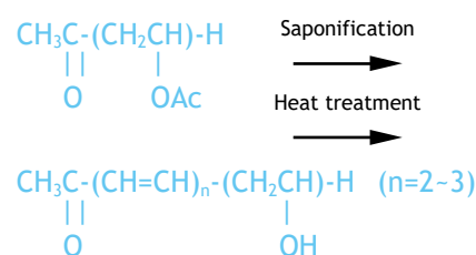
Figure 24. Double bond structure contained in PVOH
