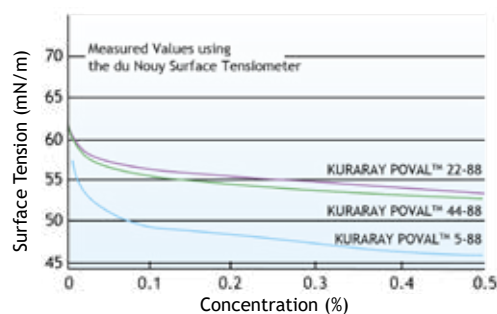
Figure 53. Surface Tension of PVOH Aqueous Solution (20°C) Influence of Degree of Polymerization
