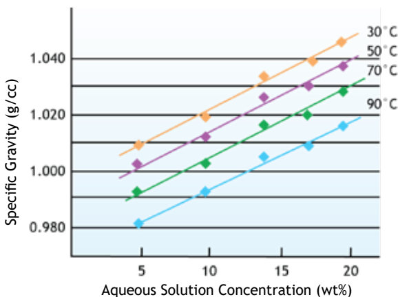
Figure 48-1. Specific Gravity of KURARAY POVAL™ 28-98 Aqueous Solution
