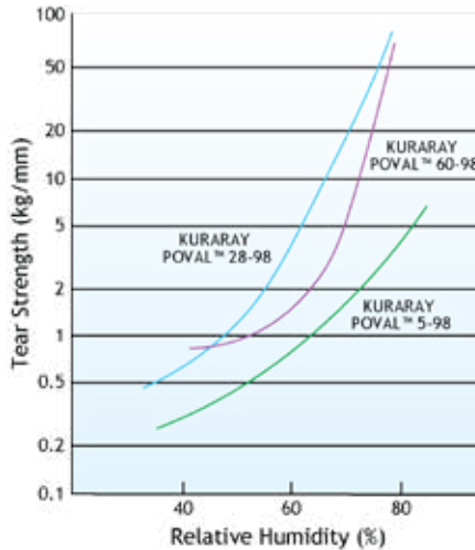
Figure 81. Tear Strength of Fully Hydrolyzed PVOH Film (20°C)
