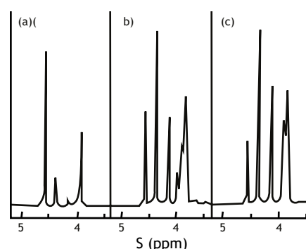
(d 6 -DMSO, 500Mz) (a) it-PVOH (mm/mr/rr=79.1/18.9/2.0) (b) at-PVOH (mm/mr/rr=22.0/48.8/29.2) (c) st-PVOH (mm/mr/rr=14.1/48.9/37.0)
