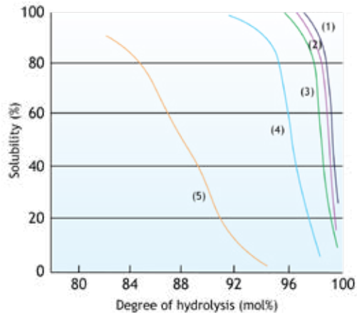
Figure 28. Influence of heat treatment on solubility of PVOH.
