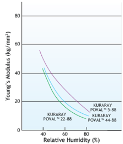
Figure 84. Young's Modulus of Partially Hydrolyzed PVOH Film (20°C)
