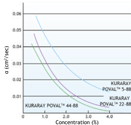
Figure 55. \alpha value of Partially hydrolyzed PVOH Aqueous Solution (20°C)
