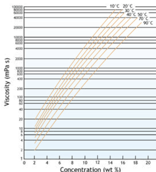
Figure 33. Relation between aqueous solution viscosity of KURARAY POVAL™ 60-98 and concentration
