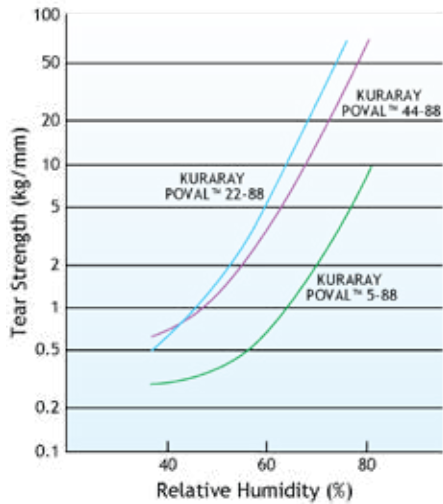
Figure 82. Tear Strength of Partially Hydrolyzed PVOH Film (20°C)
