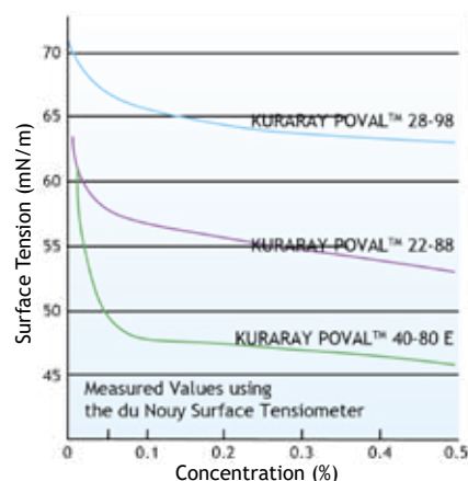
Figure 52. Surface Tension of PVOH Aqueous Solution (20°C) Influence of Degree of Hydrolysis
