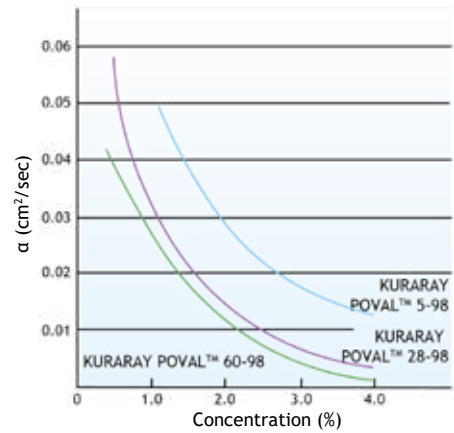
Figure 54. \alpha value of Fully Hydrolyzed PVOH Aqueous Solution (20°C)
