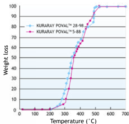
Figure 16. Thermal Decomposition of PVOH (Rate of Temperature Rise: 10°C/min, in air)
