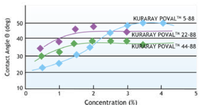
Figure 56. Contact Angle \theta of Partially hydrolyzed PVOH Aqueous Solution to Filter Paper (20°C)
