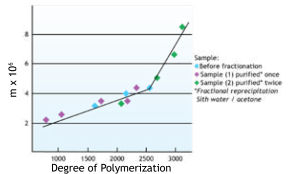
Figure 47. Relationship between Residual Acetate Group Amount and m (Concentration: 15 g/l, 30 °C)
