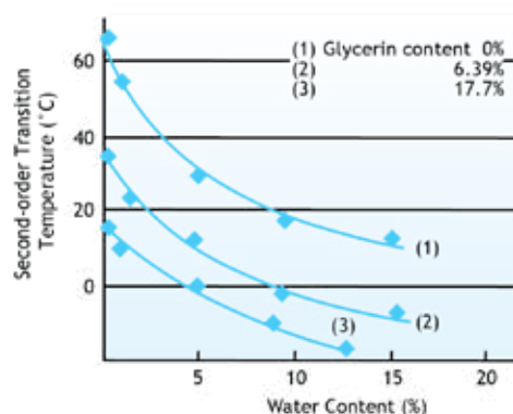
Figure 6. Synergistic Effect of Water Content and Glycerin Content on Second-order Transition Temperature of PVOH
