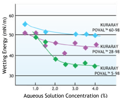
Figure 58. Wetting Energy of Fully hydrolyzed PVOH Aqueous Solution
