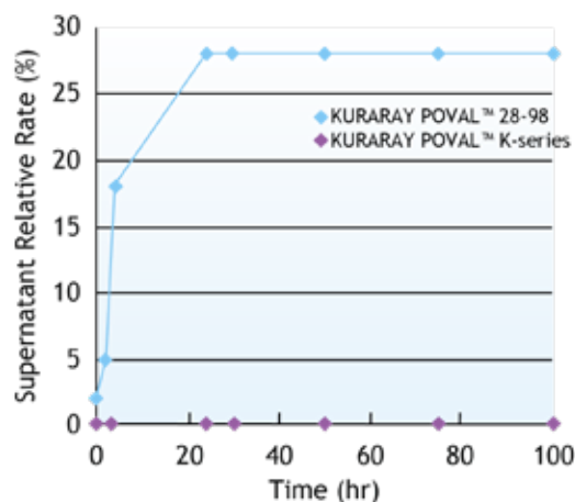
Figure 63. Compatibility of PVOH-starch Mixture (Left Stability at 50 °C)
