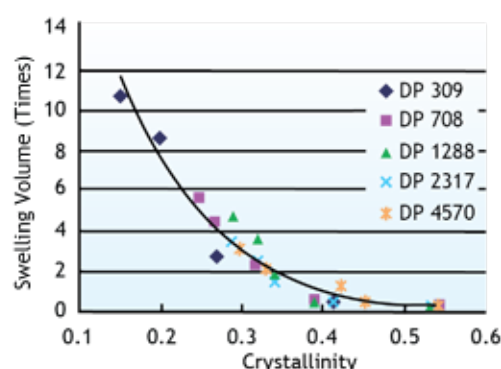
Figure 8. Crystallinity and Swelling Volume (30 °C for 48 hr)
