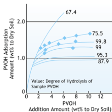
Figure 67. Adsorption Amount of PVOH to Clay* Particle (Influence of Degree of Hydrolysis) * Shokoazan Clay
