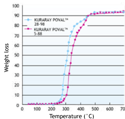
Figure 17. Thermal Decomposition of PVOH (Rate of Temperature Rise: 10°C/min, in nitrogen)
