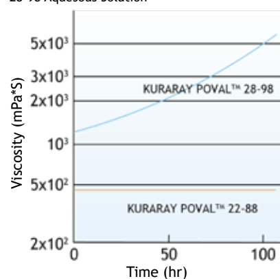
Figure 41 Viscosity Change of KURARAY POVAL™ 28-98 and KURARAY POVAL™ 22-88 with a Concentration of 8%
