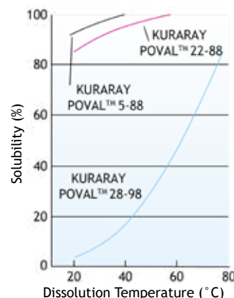
Figure 27. Solubility of Major PVOH (Influence of Dissolution Temperature)
