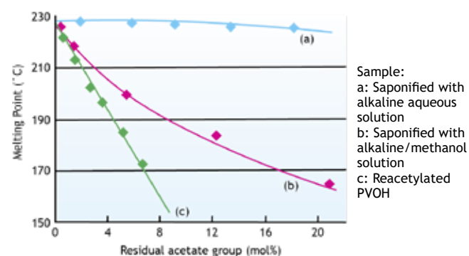
Figure 10. Influence of Residual acetate Group Amount and Its Distribution State on Melting Point of PVOH
