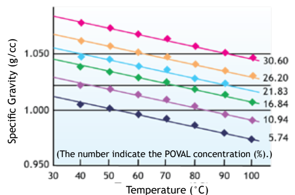
Figure 48-2. Specific Gravity of KURARAY POVAL™ 28-98 Aqueous Solution
