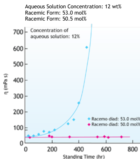
Figure 21. Temporal Change of Viscosity of PVOH Aqueous Solution with Different Stereoregularity
