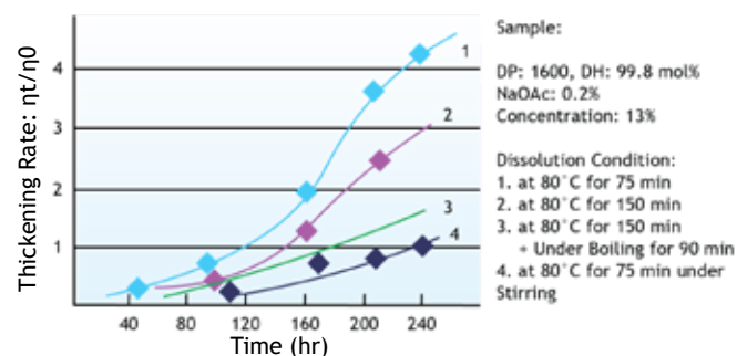
Figure 43. Influence of Dissolution Condition on Thickening of PVOH Aqueous Solution (30°C) (hr)
