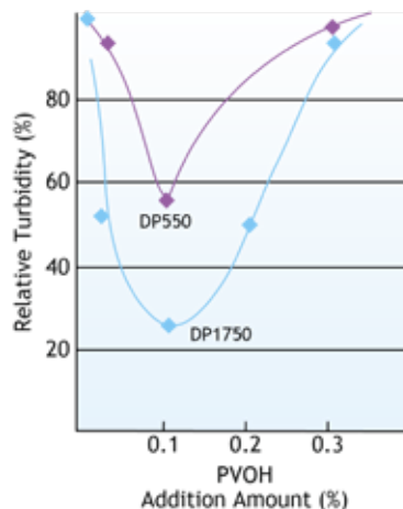
Figure 66. Influence of Degree of Polymerization of PVOH on Aggregation of Kaolin Suspension System
