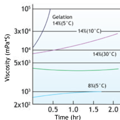
Figure 40 Viscosity Change of KURARAY POVAL™ 28-98 Aqueous Solution
