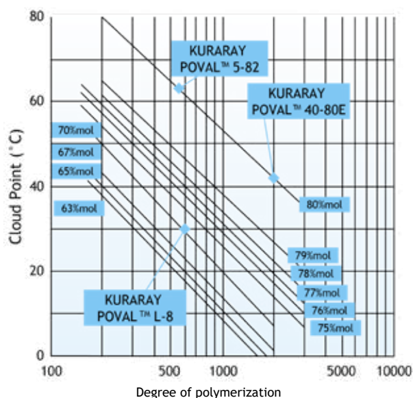
Figure 71. Influence of Degree of Hydrolysis and Degree of Polymerization on Cloud Point of PVOH Aqueous Solution (4%)
