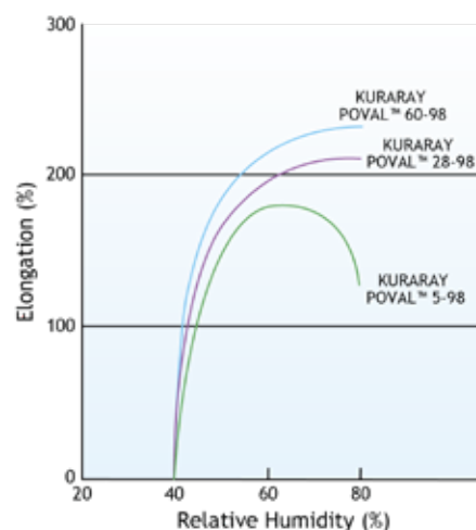
Figure 79. Elongation of Fully Hydrolyzed PVOH Film (20°C)
