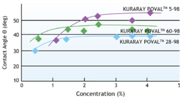
Figure 56. Contact Angle \theta of Fully hydrolyzed PVOH Aqueous Solution to Filter Paper (20°C)
