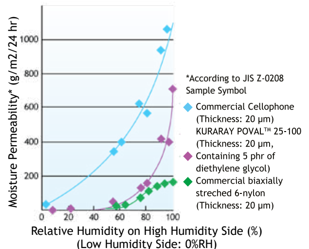
Figure 76. Moisture Permeability of Hydrophilic Polymer (35°C)
