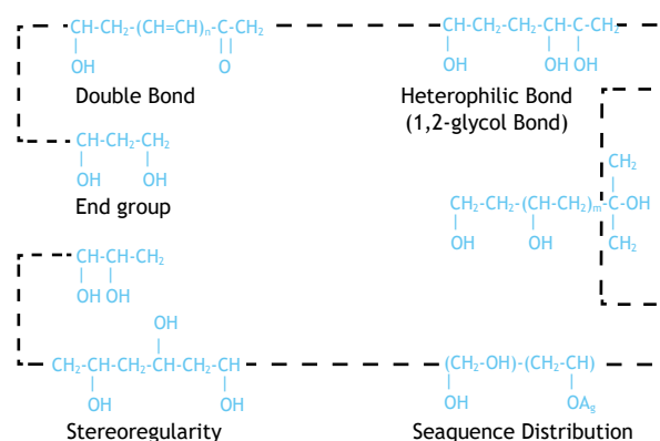
Figure 19. Primary structure of PVOH
