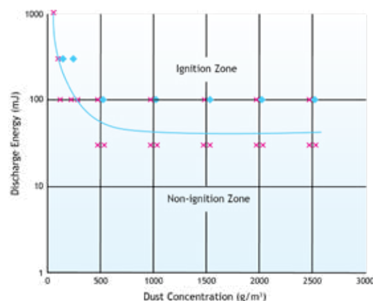
Figure 18. Relationship between PVOH Dust Concentration and Discharge Energy
