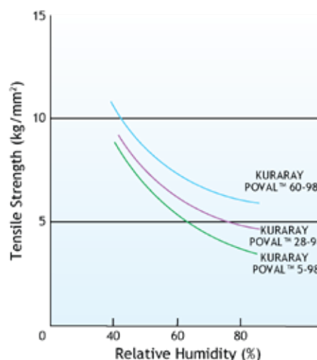
Figure 77. Tensile Strength of Fully Hydrolyzed PVOH Film (20°C)
