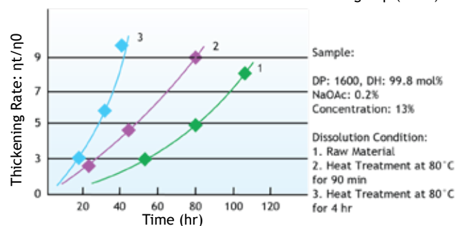
Figure 44. Influence of Heat History before Dissolution on Thickening of PVOH Aqueous Solution (30°C)
