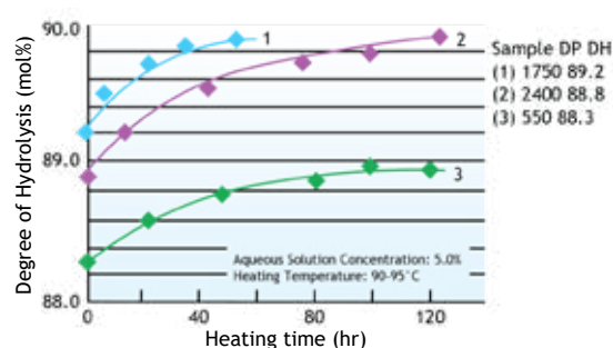
Figure 50. Change in Degree of Hydrolysis in PVOH Aqueous Solution owing to Prolonged Heating
