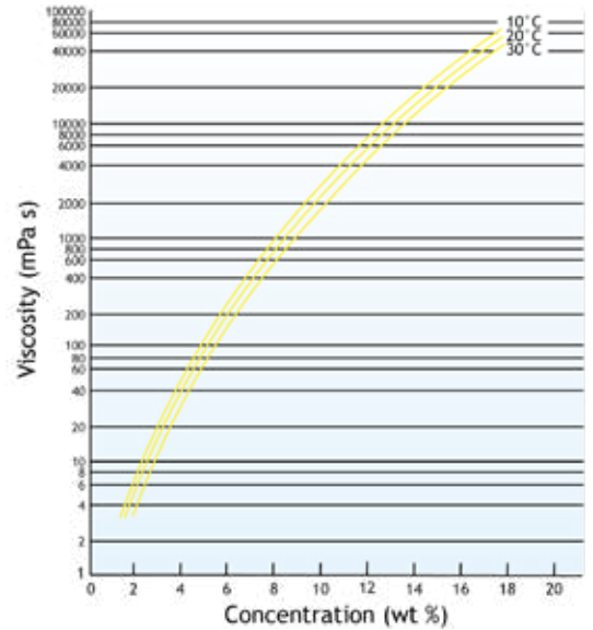
Figure 37. Relation between aqueous solution viscosity of KURARAY POVAL™ 40-80 E and concentration
