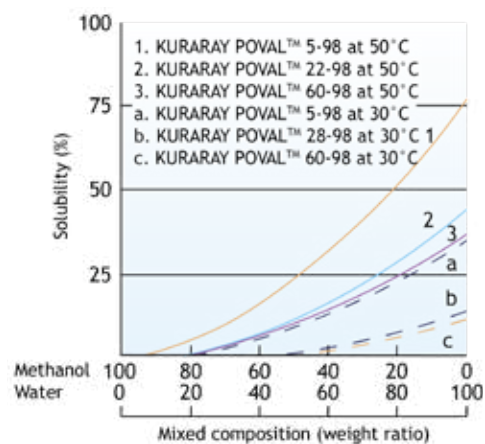
Figure 29. Solubility of fully hydrolyzed grade in water-methanol mixture
