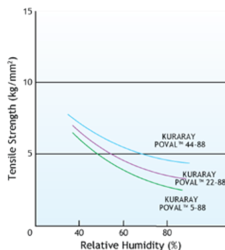
Figure 78. Tensile Strength of Partially Hydrolyzed PVOH Film (20°C) P. 31/36
