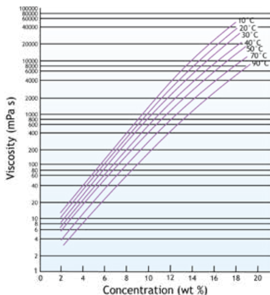
Figure 32. Relation between aqueous solution viscosity of KURARAY POVAL™ 28-98 and concentration
