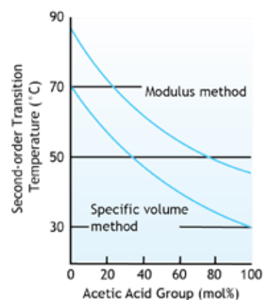
Figure 3. Second-order Transition Temperature of PVOH
