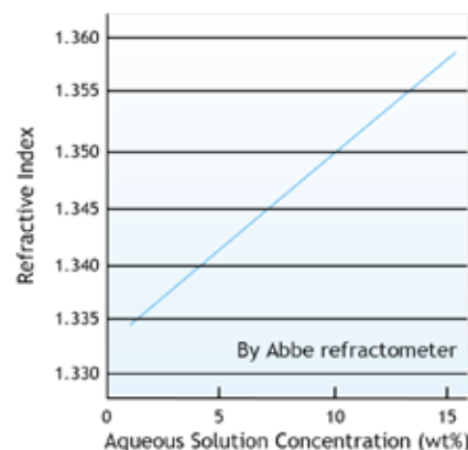
Figure 49. Refractive Index of KURARAY POVAL™ 28-98 Aqueous Solution (20°C)
