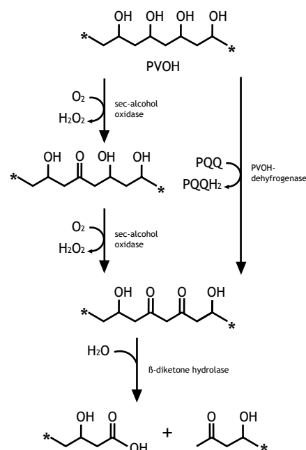
Figure 72. Biodegradation Mechanism of PVOH
