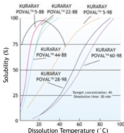
Figure 26. Solubility of Major PVOH (Influence of Dissolution Temperature)
