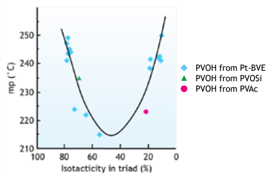
Figure 11. Relationship between Melting Point and Tacticity
