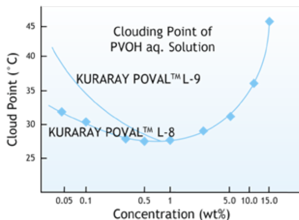
Figure 70. Correlation Example between Cloud Point and Concentration of PVOH Aqueous Solution
