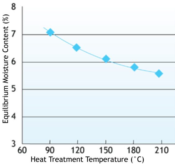
Figure 74. Influence of Heat Treatment on Equilibrium Moisture Content of PVOH Film*
