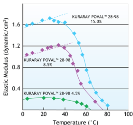
Figure 68. Relation between Temperature and Elastic Modulus of PVOH - Congo Red Gel (Congo Red Concentration: 1.5%)
