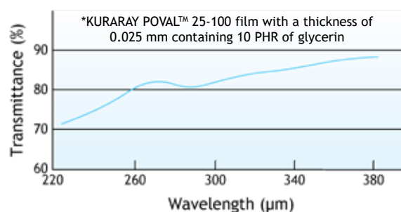
Figure 86. Ultraviolet Ray Transmittance of PVOH Film*
