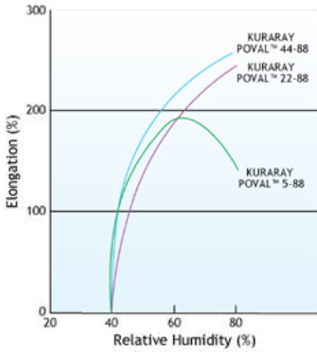
Figure 80. Elongation of Partially Hydrolyzed PVOH Film (20°C)
