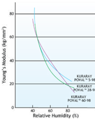
Figure 83. Young's Modulus of Fully Hydrolyzed PVOH Film (20°C)
