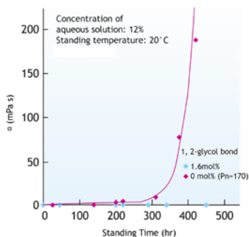
Figure 22. Temporal Change of Viscosity of PVOH Aqueous Solution with Different 1,2-glycol bond Content
