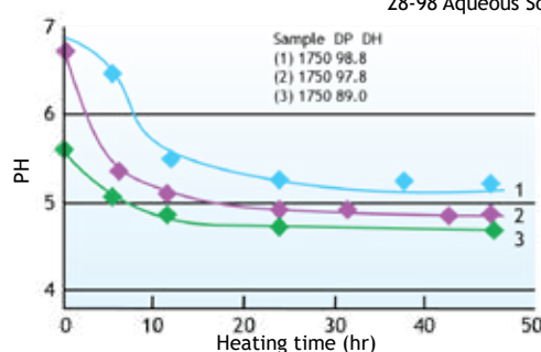
Figure 51. pH Change of PVOH Aqueous Solution owing to Prolonged Heating
