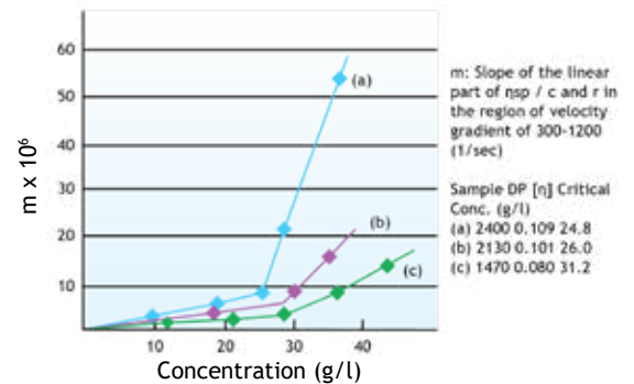
Figure 45. Relationship between m Value and Dissolution Concentration (30 °C)
