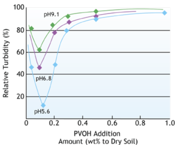
Figure 65. Aggregating and Dispersive Actions of PVOH in Kaolin Suspension System (Kaolin Concentration: 1%)
