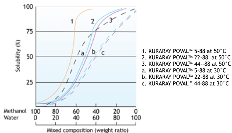
Figure 30. Solubility of partially hydrolyzed grades in water-methanol mixture
