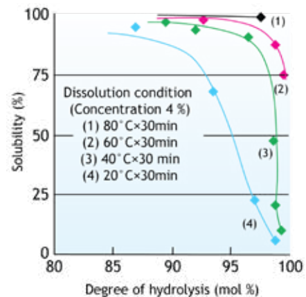
Figure 25. Influence of degree of hydrolysis on solubility of PVOH
